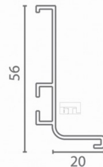
SN - 11 L Gola Profile
