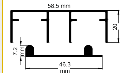
SN - 19 Double Taklu Sliding Track
