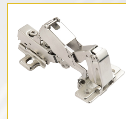
SN - 32 165° Soft Close Hinges (MS)
